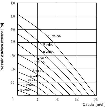
VMC EX 150
