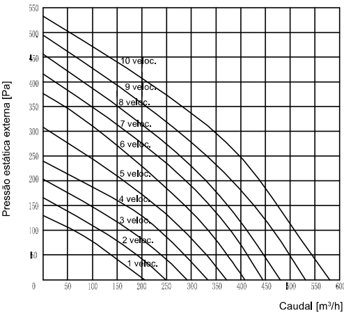
VMC EX 500
