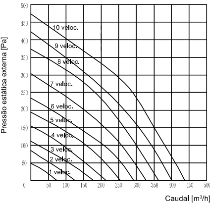
VMC EX 350
